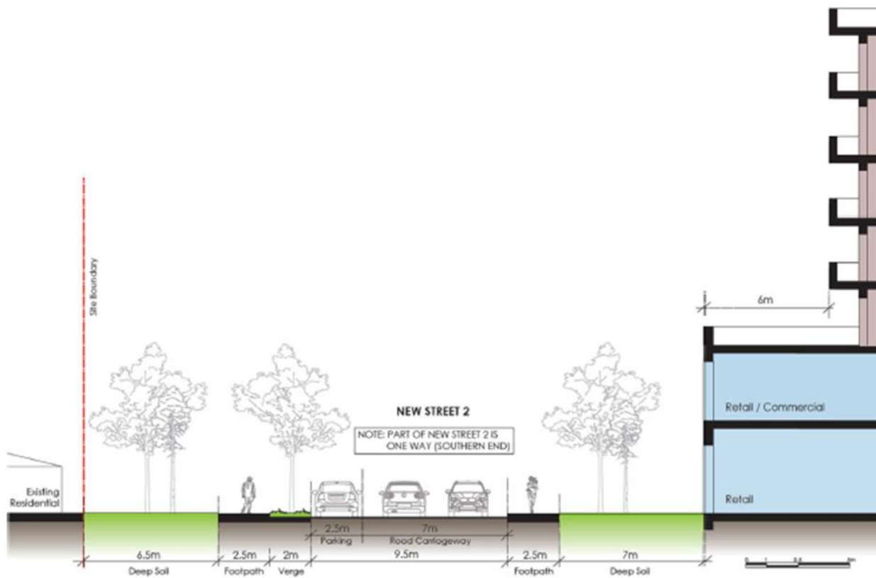
Figure 13: New Street 2 - Northern End - Section E-E
