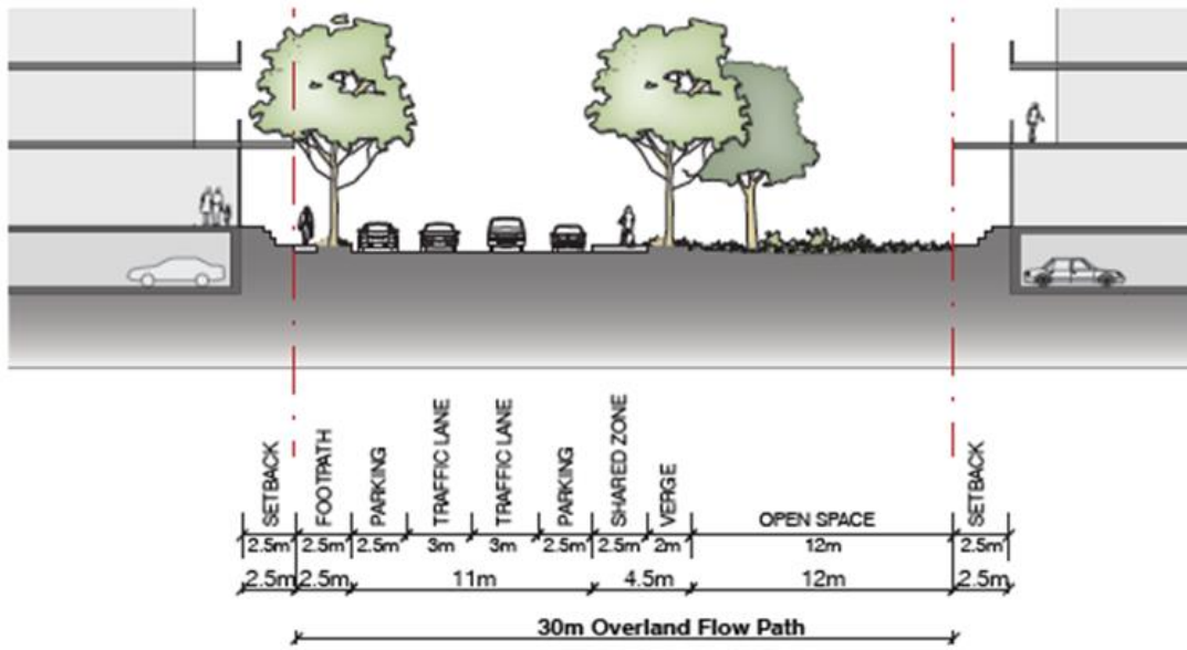
Figure 13: Section DD
