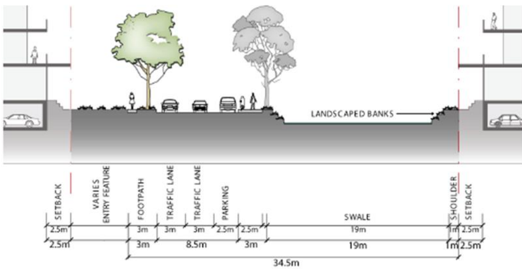
Figure 14: Section EE
