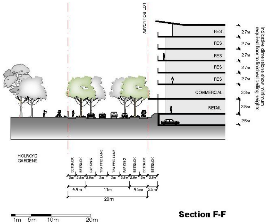
Figure 6: Section F-F
