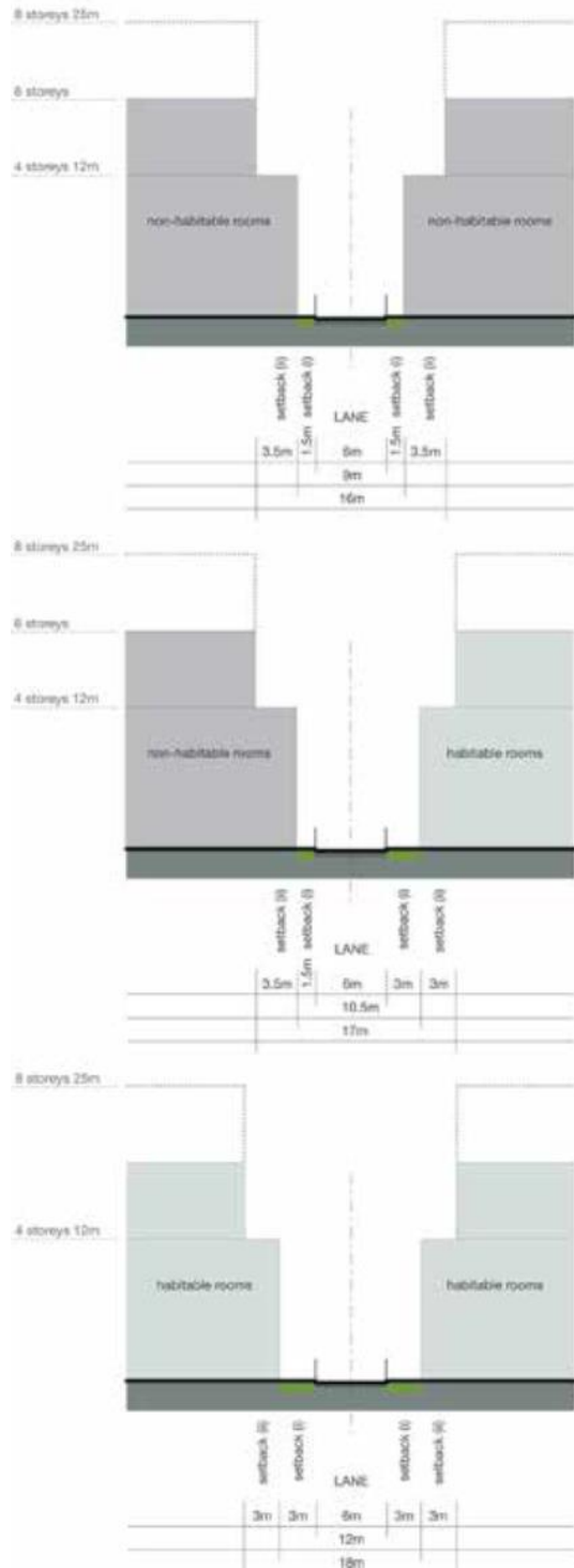
Figure 3: Lane and Street Sections
