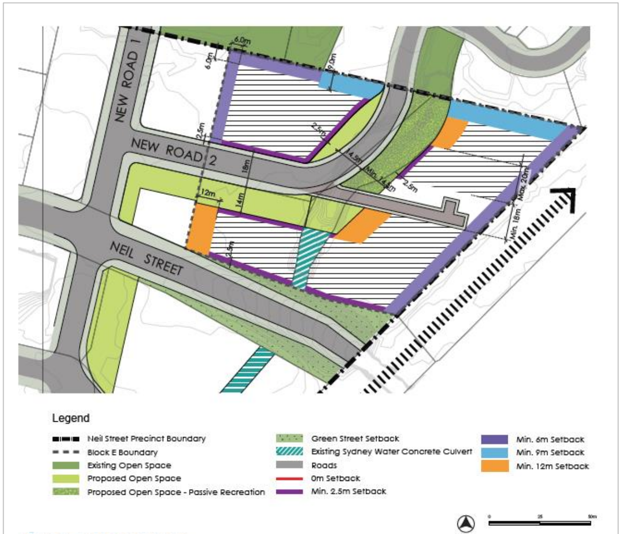
Figure 54: Block E setback plan
