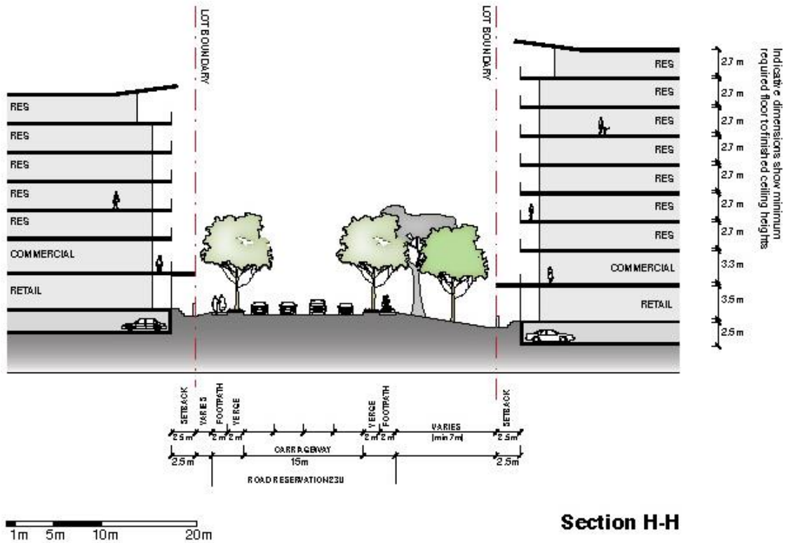
Figure 8: Section H-H
