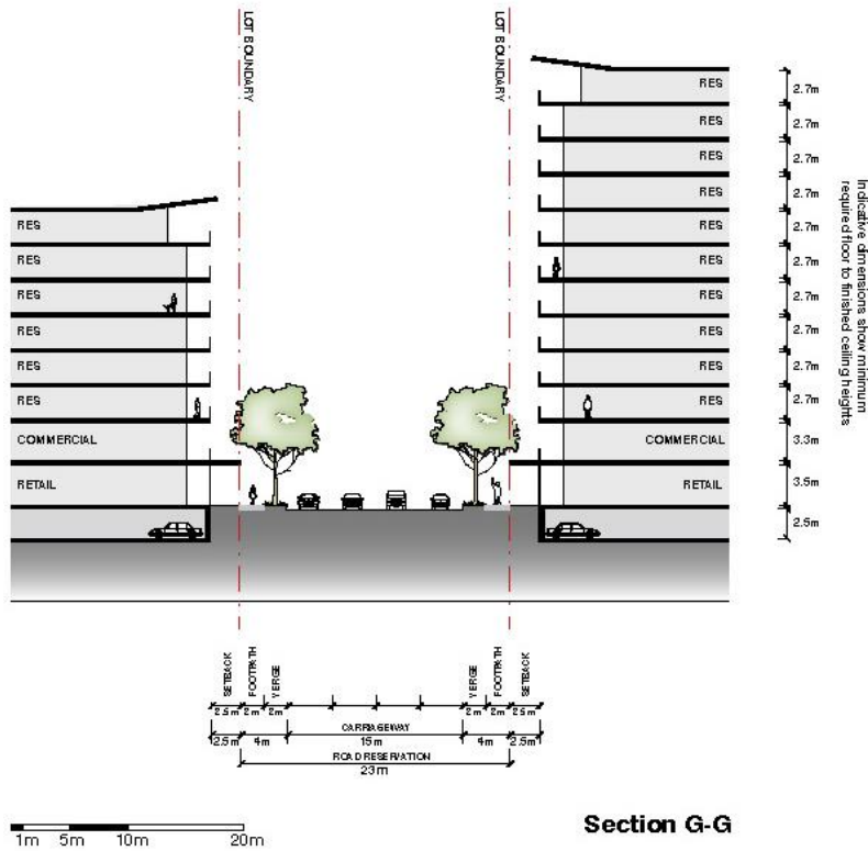
Figure 7: Section G-G
